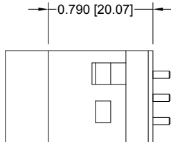
Panel Mount Male to Straight Board Mount Female
