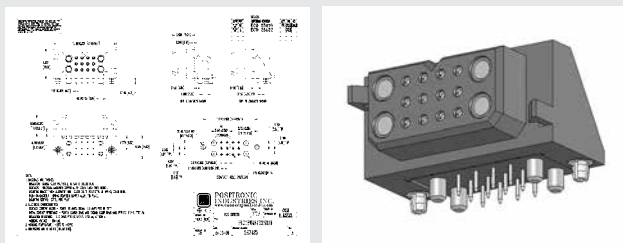
2-D Drawing
