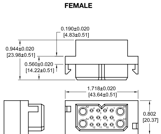
Part Number: PLC16W4F1000
