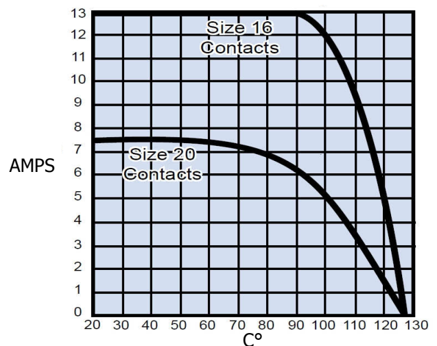
Rated Current Versus Temperature
